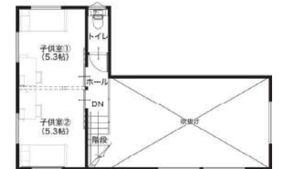
2F Plan
