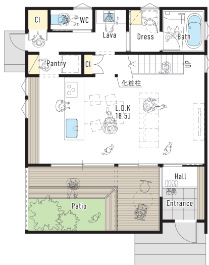
1F plan
